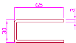
65 x 32 x 3mm STEEL GUIDE
