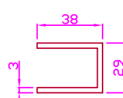
38 x 29 x 3mm ALUM GUIDE
