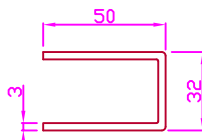
50 x 32 x 3mm STEEL GUIDE
